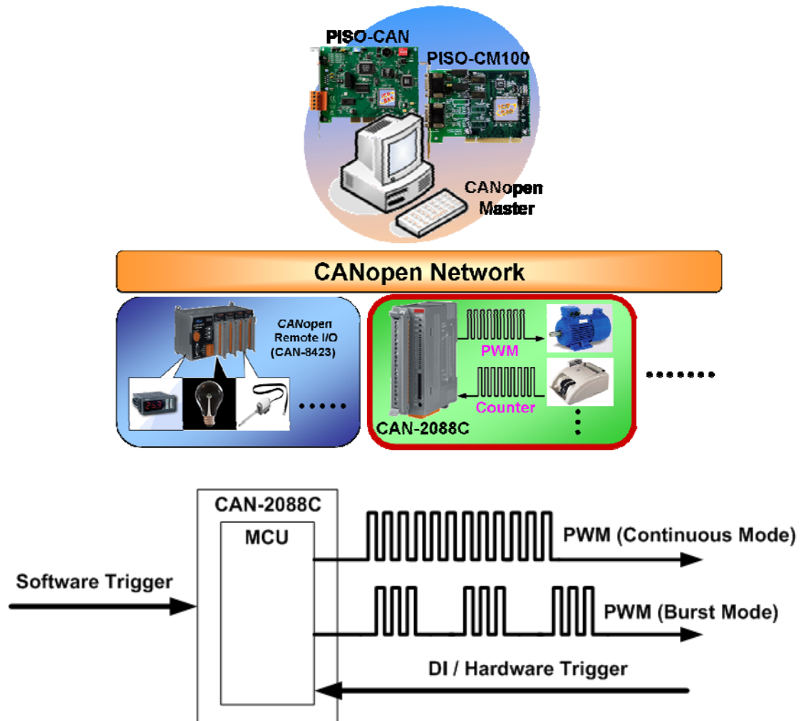
Figure 1-2 Application Structure
