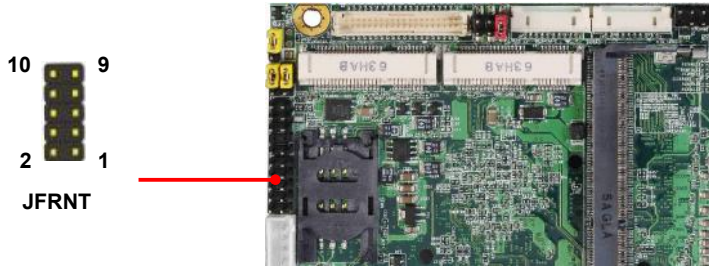
JFRNT: Front panel switch and indicator 14-pin header (Pitch 2.54mm)
