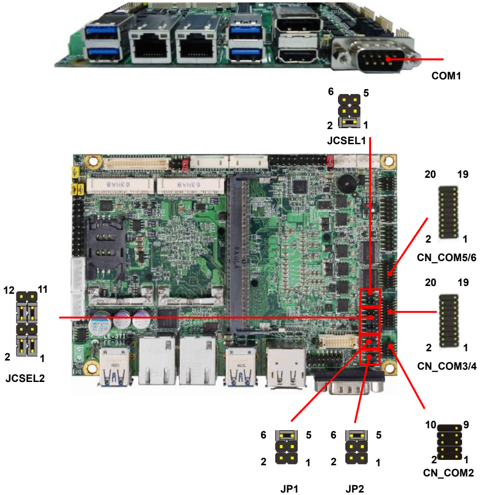
COM1: RS232 DB9 connector
