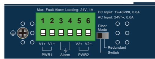
Figure 2-2: Industrial Gigabit Ethernet Switch Upper Panel
