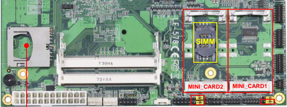
SD Slot
